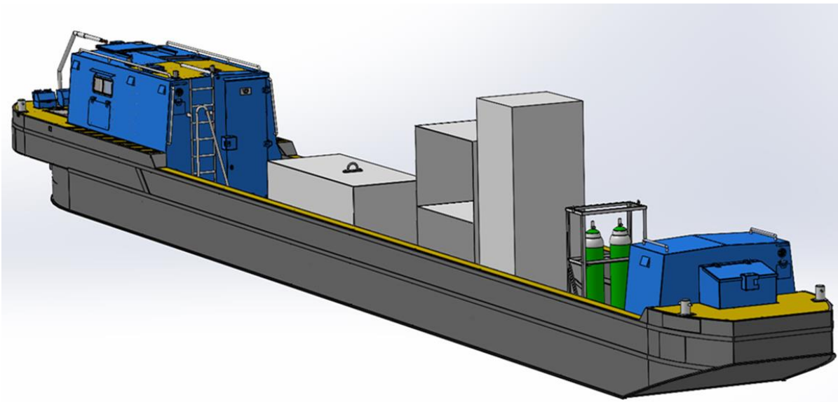
Figure 1. CRT Narrowboat schematic showing oxygen cylinders along with oxyfuel and CO2 storage system
